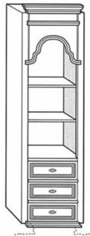
Art. 1523 Modulo Bizantino jolly 3 cass. + giorno Make-up element 3 drawers + open compart. Modul freier baustein
